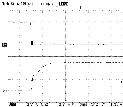
Typical Start-Up Transient with CNT AV45C-048L-050F20HAN
