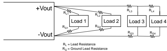
Fig.21 Mixed Power Distribution
