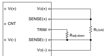
Fig.10 Circuit Configuration and Equation to Trim Up Output Voltage
